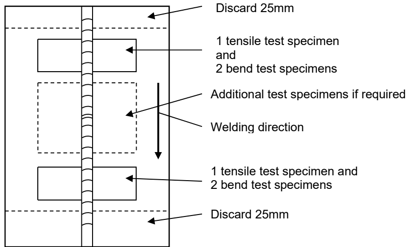
Fig.3.1.2 Location of test specimens for a butt joint in plate
