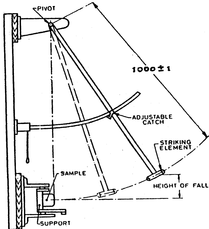
IMPACT TEST APPARTUS
