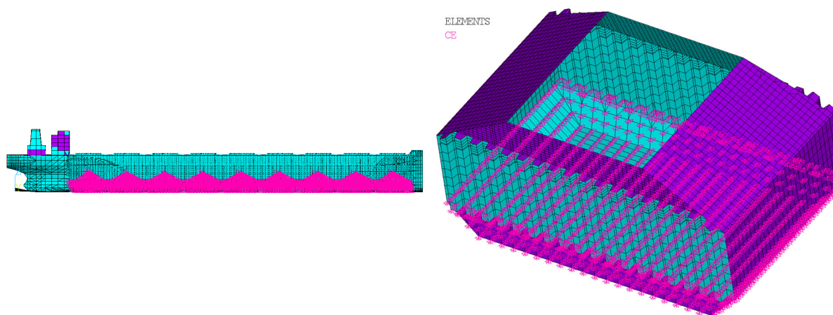
Figure 5.4.3.3.1: Illustrative distribution of cargo loads in homogeneous condition
