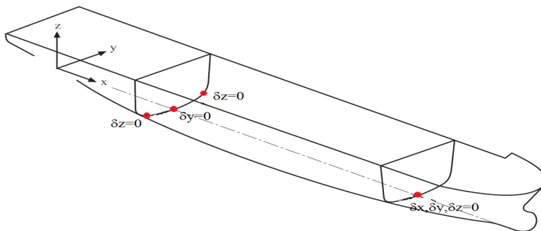
Figure 5.7.1: Boundary conditions
